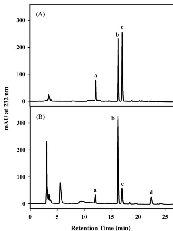
Fig. 2. SAX-HPLC analysis of CS disaccharides produced by enzymatic digestion (A) standard NZP CS; (B) ophthalmic solution; both samples (1 mg of CS/mL) were digested by chondroitinase ABC as described in the section 2.3. (a) \Delta Di-0S ( \Delta UA-[1 \rightarrow 3]-GalNAc); (b) \Delta Di-6S ( \Delta UA-[1 \rightarrow 3]-GalNAc-6S); (c) \Delta Di-4S ( \Delta UA-[1 \rightarrow 3]-GalNAc-4S); (d) \Delta Di-2,6diS ( \Delta UA-2S-[1 \rightarrow 3]-GalNAc-6S). The ophthalmic solution consists of CS, pyridoxine hydrochloride (HCl), dipotassium glycyrrhizinate, naphazoline HCl, dexpanthenol, propyl parahydroxybenzoate, cyanocobalamin, and methyl parahydroxybenzoate.
