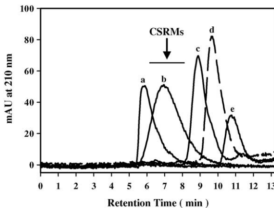
Fig. 3. MW standards and average MW range of CSRMs analyzed by HPSEC (a) CS (MW = 40,000 Da); (b) CS (MW = 15,000 Da); (c) aacharan sulfate oligosaccharides ( n=15 , MW = 6975 Da); (d) aacharan sulfate oligosaccharides ( n=10 , MW = 4530 Da); (e) aacharan sulfate oligosaccharides ( n=5 , MW = 2265 Da). The bar indicates the range of retention time of CSRMs.
