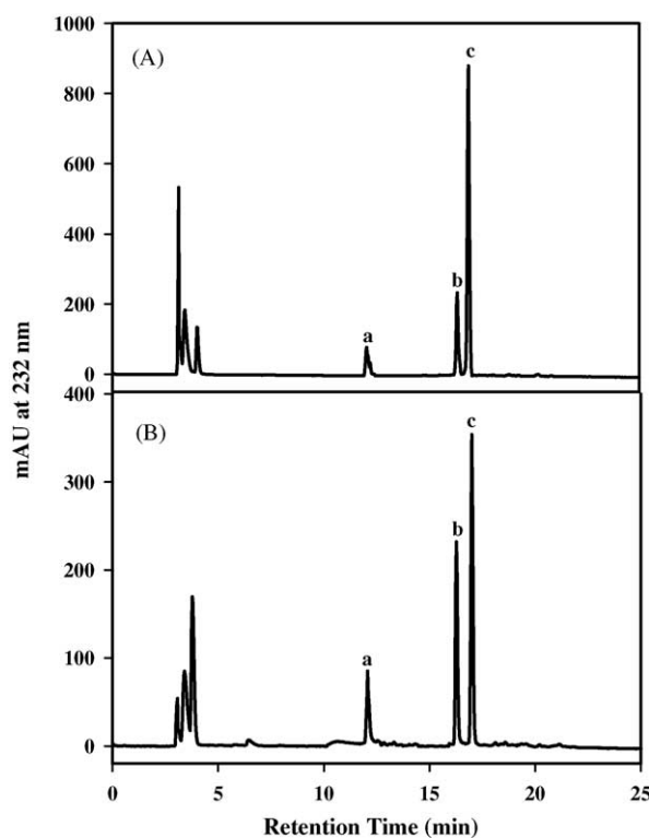
Fig. 4. SAX-HPLC analysis of the disaccharides derived from CS in soft capsules and liquid preparations after pretreatment (A) soft-capsules; (B) liquid preparations; both samples were digested by chondroitinase ABC after pretreatment as described in the section 2.6. (a) \Delta Di-0S ( \Delta UA-[1→3]-GalNAc); (b) \Delta Di-6S ( \Delta UA-[1→3]-GalNAc-6S); (c) \Delta Di-4S ( \Delta UA-[1→3]-GalNAc-4S). The soft capsule contains CS, tocopherol acetate, fursultiamine, nicotinamide, pyridoxine HCl, pantothenic acid, riboflavin butyrate, \gamma -oryzanol, cyanocobalamin, methyl parahydroxybenzoate, propyl parahydroxybenzoate, garlic extract. The liquid preparations contain CS, pyridoxine HCl, cyanocobalamin, nicotinamide, sodium pantothenate, thiamine HCl, carnitine HCl, anhydrous caffeine, riboflavin sodium phosphate, diluted ethanol extract of Ginseng Radix and Oriental Bezoar, Royal Jelly, Epimedium Herba extract, sodium benzoate, and propyl parahydroxybenzoate.
